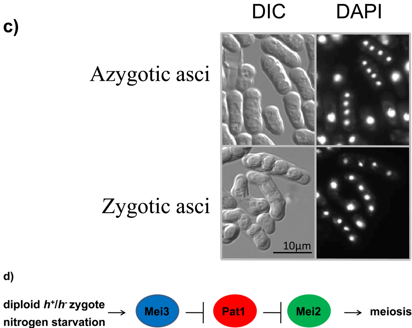
Figure 1. Zygotic and azygotic meiosis in the fission yeast S. pombe
