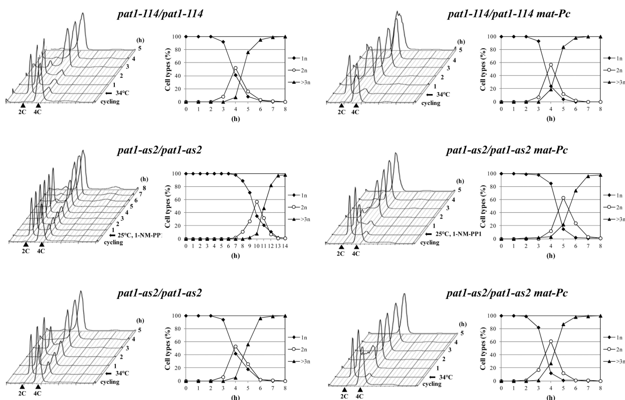
Figure 2. Synchronous meiosis induced by inactivation of Pat1
