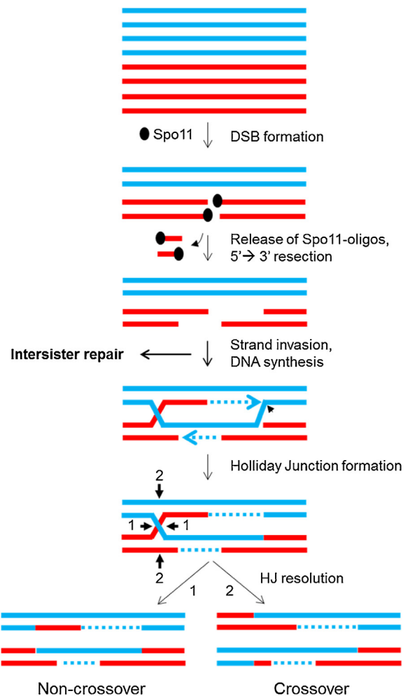
Fig. 1. Formation of crossovers and non-crossovers at Spo11-induced DSBs. Red and blue lines are single DNA strands, and each pair depicts one sister chromatid of each homologous chromosome (the non-interacting sisters are shown only in the top panel); dotted lines are DNA synthesized during DSB repair. After meiotic replication, Spo11 or its ortholog induces DSBs and covalently attaches to the 5' ends. Spo11 is then cleaved from the ends by an endonuclease to release a short oligonucleotide attached to Spo11. The 5' ends are further resected to generate long 3' overhangs, which invade intact duplex DNA, either the homolog or the sister chromatid; this side reaction with the sister produces no genetic recombinants. Holliday junctions, either single (shown) or double (not shown), are formed and then resolved into either crossovers or non-crossovers (respectively with the non-parental or parental DNA configuration flanking the region of DNA exchange). These reactions have been demonstrated by direct DNA analysis in budding and fission yeasts and are inferred, from genetic and cytological data and limited DNA analysis, to occur in other species. In an alternative to Holliday junction formation, strand invasion at the third step can prime limited DNA synthesis; the unwound product can anneal with the other initially broken DNA end and produce a non-crossover. This proposed reaction is called synthesis-dependent strand-annealing.
