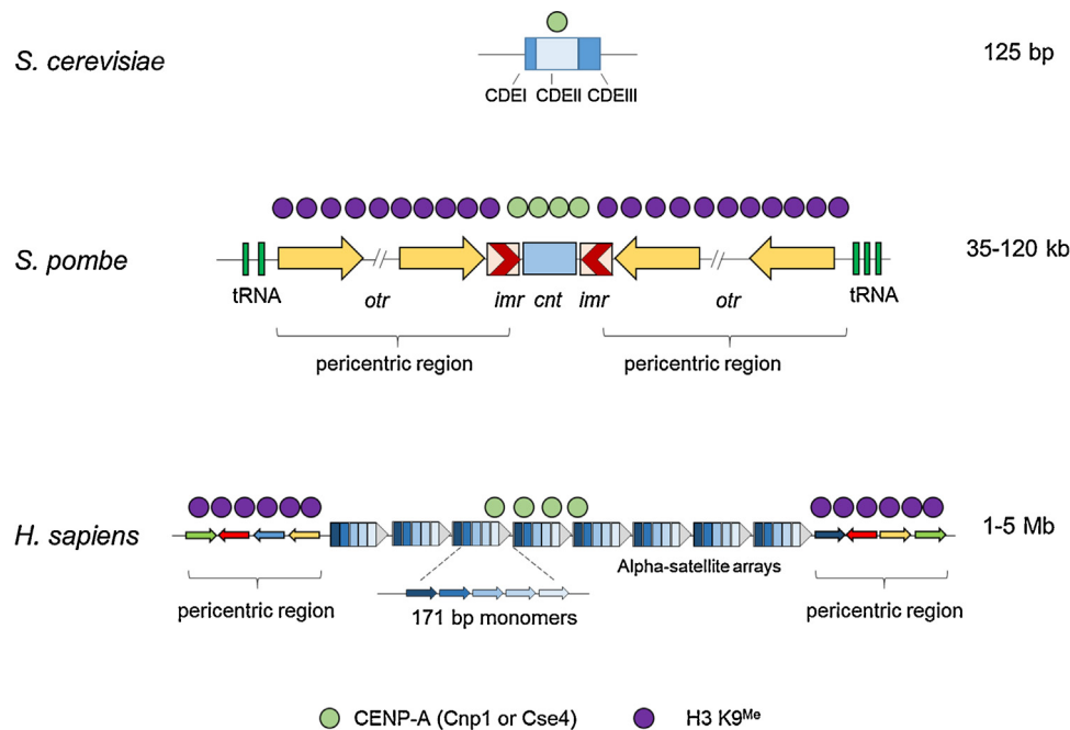
Fig. 4. Structure of centromeres in yeasts and humans. The budding yeast S. cerevisiae has 125 bp (“point”) centromeres with three conserved regions—CDEI, II and III. A single nucleosome containing the centromere-specific histone H3 variant Cse4 (CENP-A in most other organisms) occupies the whole centromere. The fission yeast S. pombe contains large 35–120 kb (“regional”) centromeres consisting of a central core ( cnt ) surrounded by innermost repeats ( imr ) and outermost repeats ( otr ). The central core contains nucleosomes with CENP-A (Cnp1 in S. pombe ), while the inverted repeats bear H3 K9me histones that form the pericentric heterochromatin. Human centromeres have large 1–5 Mb arrays of repetitive DNA consisting of 171 bp alpha-satellite repeats as the basic repeating unit. An array consists of multiple copies of higher order repeats which themselves are made up of multiple alpha-satellites that are diverged from each other. These arrays contain CENP-A interspersed with H3 K4me histones. The pericentric region contains stretches of monomeric alpha-satellite repeats that are in random orientation and are bound by H3 K9me histones that form the heterochromatin. The complete organization of human centromeres is still being worked out, and the schematic shown here is a model based on current understanding.
