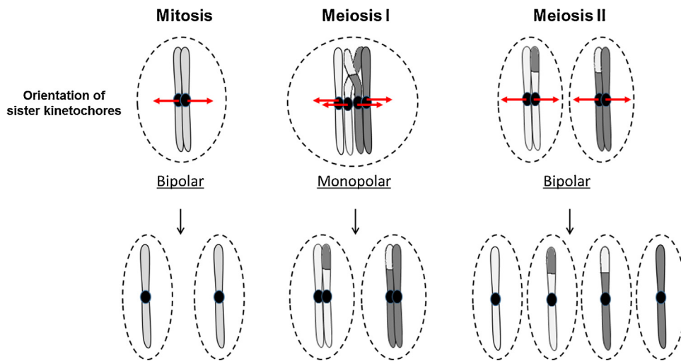
Fig. 2. Orientation of kinetochores during mitosis and meiosis. In mitosis, kinetochores attach to the centromeres of the sister chromatids, orient toward opposite poles (bipolar orientation), and segregate into separate daughter nuclei. During the first meiotic division, however, both sister kinetochores orient toward the same pole (monopolar orientation) and segregate into the same daughter nucleus. Proper direction of segregation is ensured by sister chromatid cohesion and the tension generated due to crossovers (light grey–dark grey junction) between homologs. This reductional division results in separation of the homologous centromeres and the attached chromosomal arms and reduces the number of chromosomes by half. The second meiotic division is similar to mitosis, and bipolar orientation of the sister kinetochores results in separation of the chromatids into four haploid nuclei.
