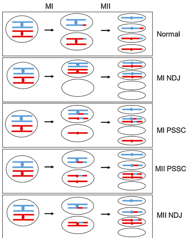
Fig. 3. Meiotic chromosomal missegregation resulting from pericentric crossovers. Red and blue lines depict homologs (duplex DNA); red and blue dots depict centromeres. Crossovers, depicted by red-blue junctions, in chromosomal arms are essential for proper segregation of chromosomes during meiosis, but crossovers too near the centromere are harmful. Normally during MI, the centromeres of homologs with their attached chromosomal arms segregate to opposite poles, whereas in MII the sister centromeres segregate to opposite poles, giving rise to four haploid nuclei. During non-disjunction (NDJ) of homologs in MI, which primarily arises due to lack of crossovers in the arms, both homologs migrate to the same pole and then segregate properly at MII, giving rise to two nullisomes (nuclei lacking a chromosome) and two disomes (nuclei with two chromosome copies). Precocious separation of sister chromatids (PSSC) occurs when cohesion is lost between the sister chromatids and can occur in either MI or MII. Crossovers too close to the centromeres (pericentric crossovers) are associated with such PSSC events. In MI PSSC, sister centromeres of one homolog segregate to opposite poles at MI followed by proper MII, giving rise to a nullisome and a disome containing homologous centromeres. In MII PSSC, sisters go to the same nucleus at MI but missegregate at MII, giving rise to a nullisome and a disome containing sister centromeres. MII NDJ has proper MI but aberrant segregation at MII, resulting in a fate similar to MII PSSC. These aberrant events are also linked to the presence of pericentric crossovers. Some of these missegregation events give rise to similar types of aneuploids, but careful tetrad analysis with multiple markers can distinguish them.
