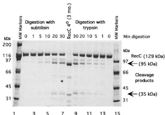
FIGURE 6.—Physical evidence for two RecC domains. Purified RecC polypeptide (2 \mu g per lane) was digested with subtilisin (lanes 2–7) or trypsin (lanes 9–14) for the times indicated. Lanes 1 and 15 contained size markers (Bio-Rad) and lane 8 contained RecC polypeptide that was stored for several months at 4°. The digestion products were analyzed by gel electrophoresis and visualized by staining (Fast stain, Zoion Research).
