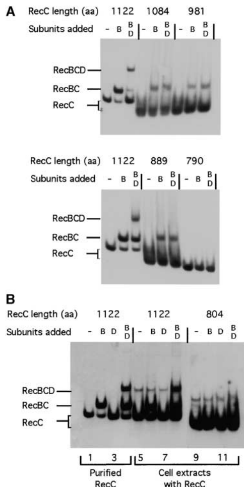
FIGURE 5.—C-terminal deletions of recC fail to assemble RecD into holoenzyme. Extracts were prepared as described in Figure 2 from V330 [ \Delta(recC\text{-argA})234 ] containing plasmids expressing full-length RecC (A, pSA125; B, pSA161) or the indicated C-terminal deletions. Purified RecB polypeptide or extract containing RecD polypeptide, or both, were added to the RecC extract as indicated, and assembly of heterodimer and heterotrimer forms of RecBCD enzyme were monitored on native polyacrylamide gels as in Figure 2A.
