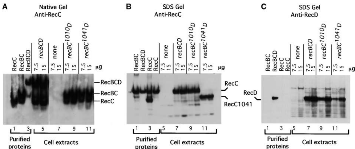
FIGURE 2.— RecC † mutants do not assemble RecD into RecBCD enzyme heterotrimer. Extracts were from late log phase cultures of strain V330 [ \Delta ( recC-argA )234] containing derivatives of plasmid pDWS2 ( recBCD ), pAC2 ( recBC 1010D ; AMUNDSEN et al. 1986), or pSA160 ( recBC 1041D ). Purified RecC, RecBC, and RecBCD enzyme (40 ng each) were run as markers. Forms of RecBCD enzyme contained in 7.5 or 15 \mu g of extract protein were separated on native or SDS polyacrylamide gels and detected by Western analysis using the indicated monoclonal antibodies. The RecC polypeptide shown in lane 3 of part B had been stored at 4° for several months and contained an apparent protease cleavage product (see RESULTS).
