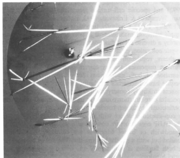
Fig. 2. Crystals of dimeric NGAL, photographed through crossed polarizers, grown from PEG at low pH. Average crystals grow to lengths of between 400 and 700 \mu\text{m} with widths of up to approximately 25 \mu\text{m} .
