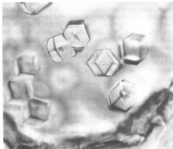
Fig. 1. Crystals of monomeric NGAL grown from PEG/ammonium sulfate. Average crystal dimensions are approximately 350 \times 350 \times 350 \mu\text{m} .
