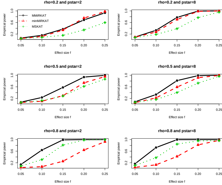
Figure 2: Empirical powers of MMiRKAT, minMiRKAT and MSKAT under n = 1000 . \circ , \triangle and + represent MMiRKAT, minMiRKAT and MSKAT respectively.
