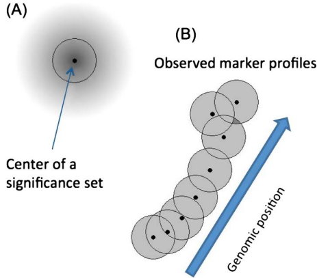
FIG. 1. A two-dimensional schematic representation of the geometric interpretation of permutation p -value, reflecting genotype profiles that actually reside in 2^n -space. (A) In the general situation, the function P(r, \alpha) , shown in grayscale, decreases with distance from the center of a significance set. Under hypersphere assumption, P(r, \alpha) is either 0 or 1, thus, it can be illustrated by a hypersphere surrounding the center of the significance set. (B) The space occupied by the series of markers is calculated serially. Denote the neighborhood region of the h th marker as B_h . Then the contribution of the h th marker to \Psi(r_\alpha) is approximated by B_h \setminus (B_h \cap B_{h-1}) , where “ \setminus ” indicate set difference. As indicated by the darker shade, this serial counting approximation is not exact when (B_h \cap B_k) \notin (B_h \cap B_{h-1}) , for any k < h - 1 . Note the dot in (A) is the center of a significance set, while the dots in (B) are the observed marker genotype profiles.
