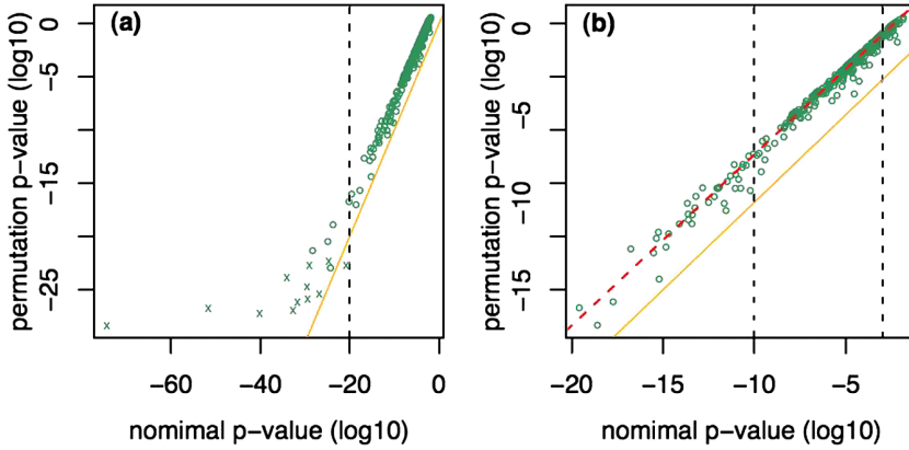
FIG. 4. Comparison of permutation p -value estimates and nominal p -values. (a) Scatter plot of permutation p -value estimates vs. nominal p -value in \log_{10} scale for the 500 gene expression traits. Those unreliable permutation p -value estimates are indicated by “x.” See footnote 2 for explanation. (b) Scatter plot for 483 gene expression traits with nominal p -value larger than 10^{-20} . In both (a) and (b) the solid line is y = x . In (b), the broken line fitting the data is obtained by median regression for those 359 genes with nominal p -values between 10^{-10} and 10^{-3} .
